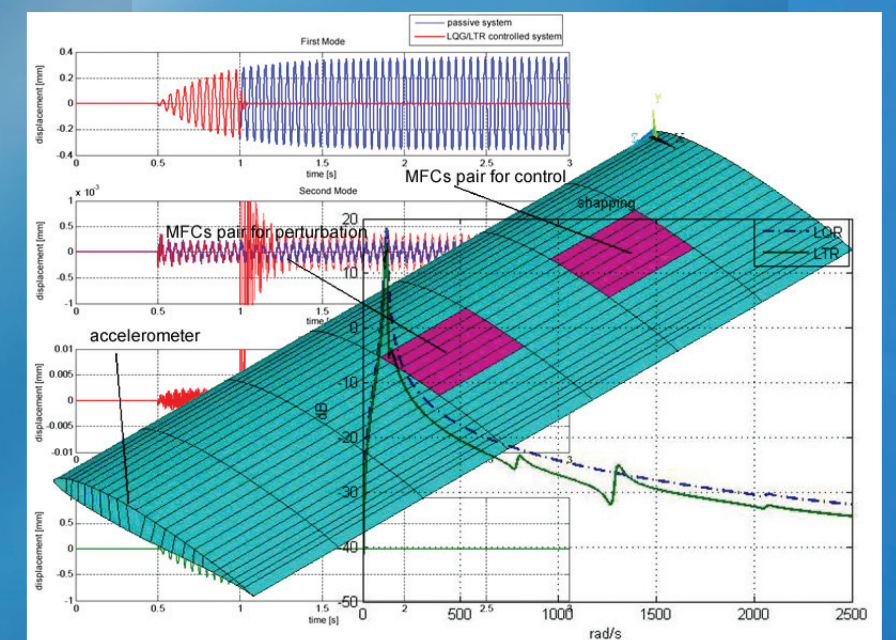
System for structural health monitoring and active vibration control
